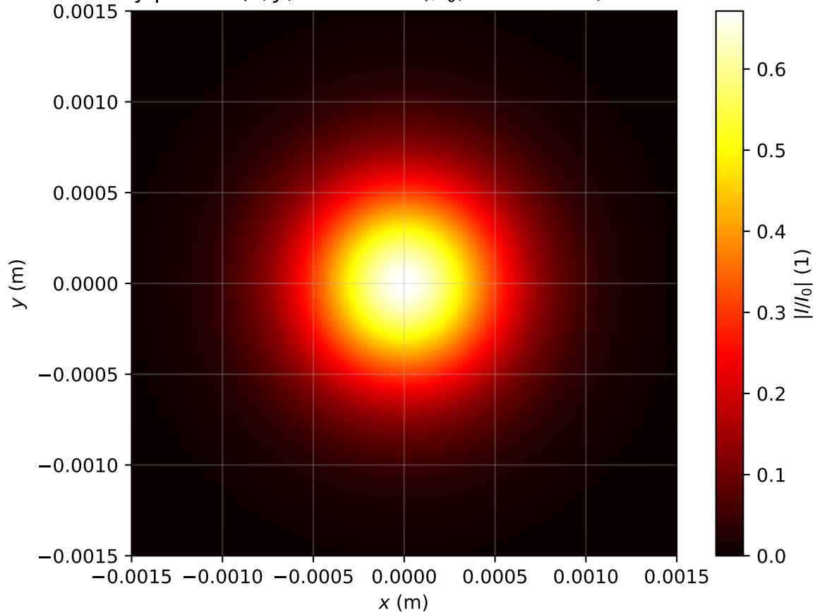
Intensity profile I(x, y, z = 3.025m)/I_0 , \text{Pin}=0.6\text{Pcr} , artificial time
